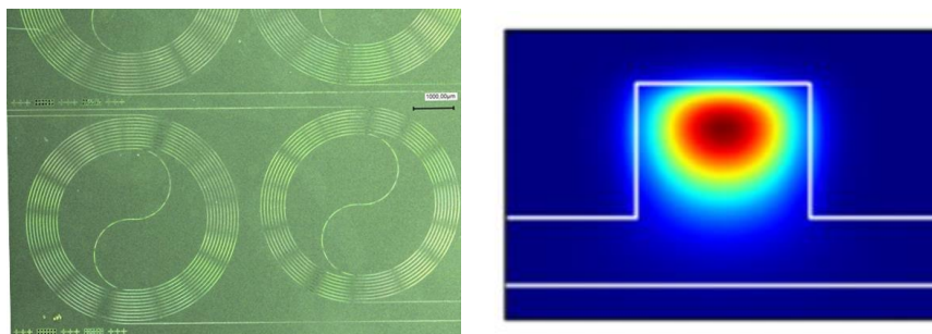
Fig. 1: left: picture of integrated mid-IR photonic integrated circuit based on Ge-rich SiGe platform / right: optical mode calculation showing the strong confinement of light in the core of a graded waveguide.
